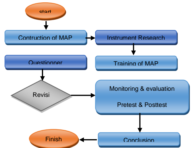
Gambar 1. Alur penelitian
